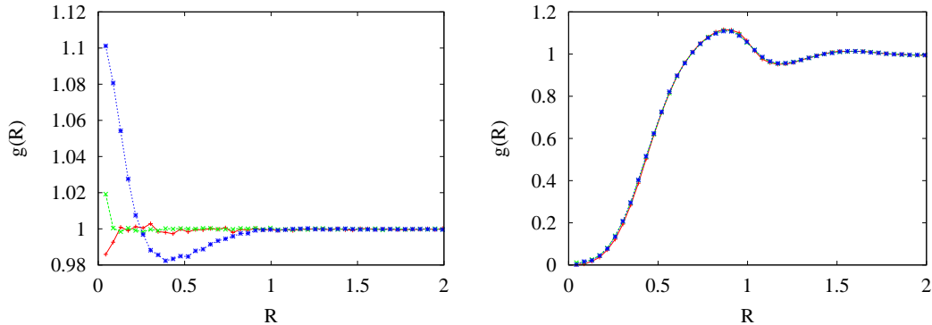
Fig. 1. Radial distribution function for three integrator methods. Velocity Verlet with star symbols (*), Shadlow scheme with ( \times ) symbols and Trotter DPD with (+) symbols. Left figure corresponds to an ideal gas simulation a_{kl} = 0 . Right figure corresponds to simulations including conservative forces with a_{kl} = 25 .
